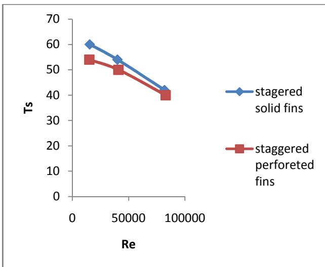
Fig. 7: Reynolds number V/s Surface temperature
