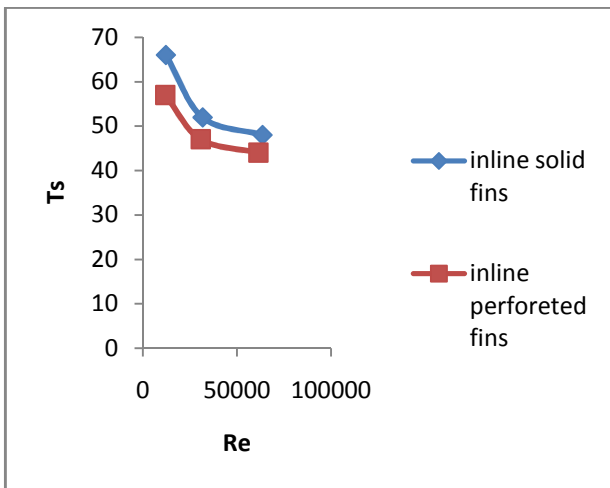
Fig.6: Reynolds number V/s Surface temperature
