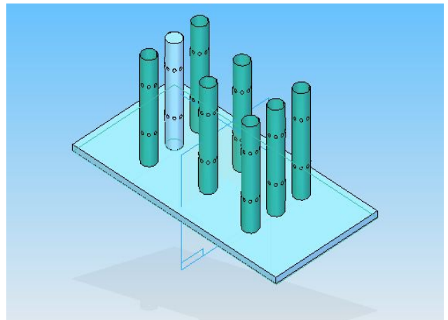
Fig.5: Staggered arrangement of Fin with perforations
