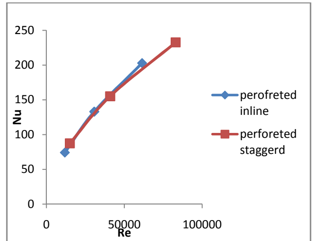
Fig.8: Reynolds number v/s Nusselt number
