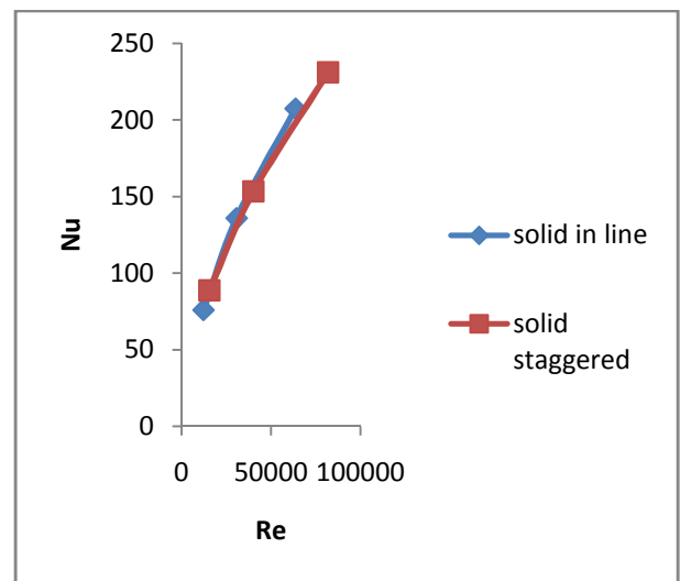
Fig.9: Reynolds number v/s Nusselt number
