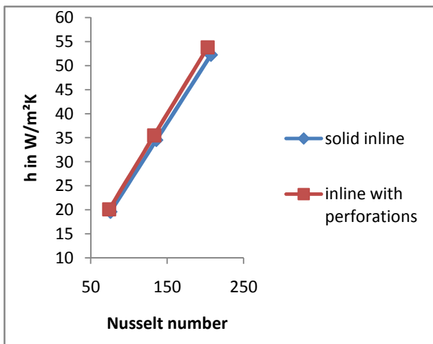
Fig.10: Nusselt Number vs. heat transfer coefficient
